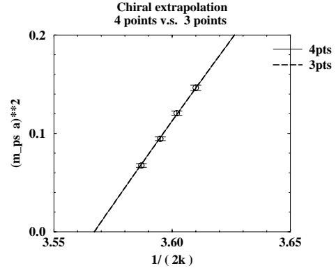
Figure 2. The Chiral extrapolation of m_{PS}^2 for \beta = 5.9 . The four \kappa fit (solid line) and the three \kappa fit (dashed line) are almost indistinguishable.
